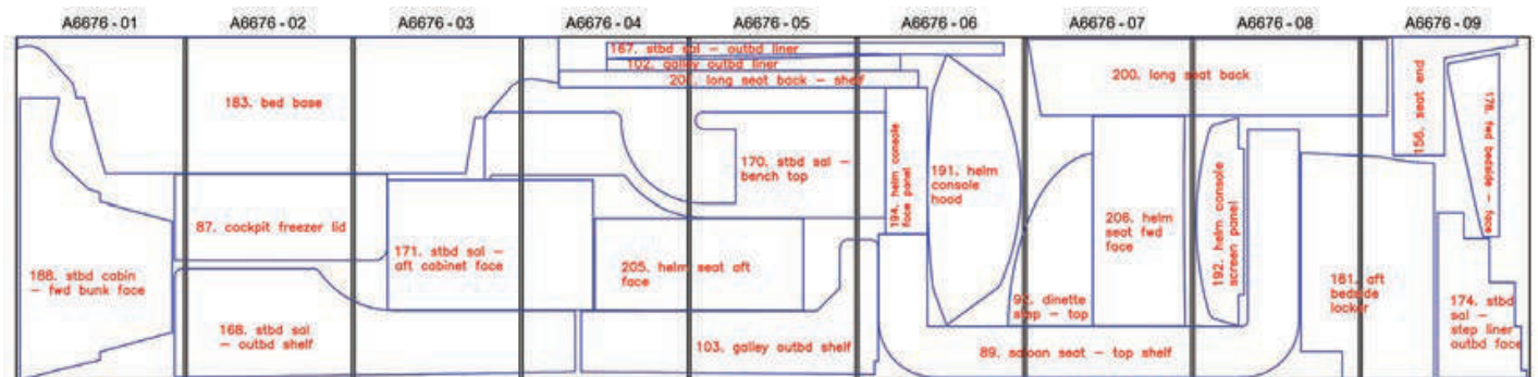
NESTING EXAMPLE - MARINE BULKHEADS AND CABINERY
