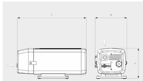
Dimensional drawing — L 499 x W 253 x H 246 mm
