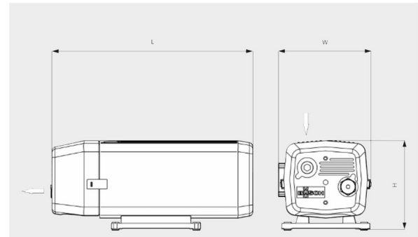
Dimensional drawing — L 554 x W 257 x H 246 mm
