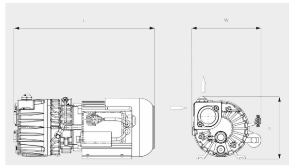
Dimensional drawing — L 248 x W 172 x H 141 mm
